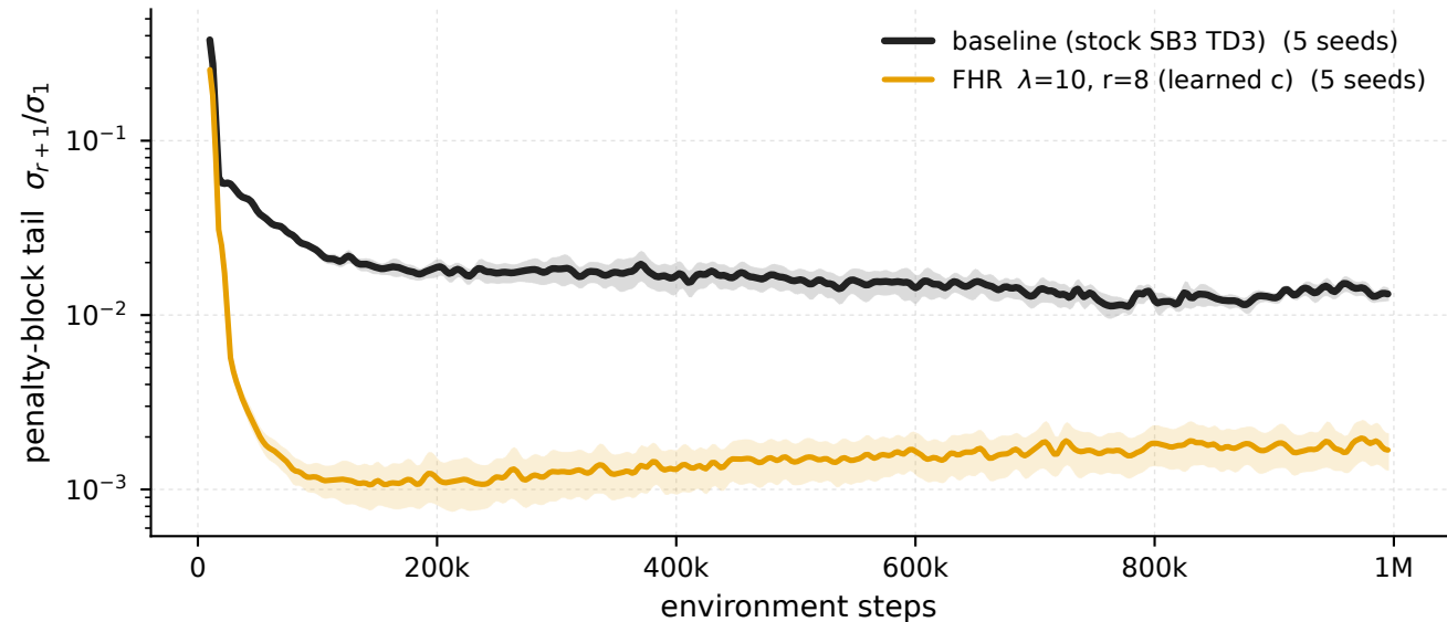
Ant-v5 - \lambda 10 \cdot r 8 vs baseline, penalised windows penalty-block tail \sigma_{r+1}/\sigma_1
