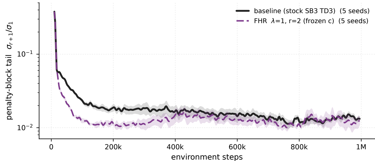
Ant-v5 - \lambda 1 \cdot r 2 frozen-c vs baseline, penalised windows penalty-block tail \sigma_{r+1}/\sigma_1
