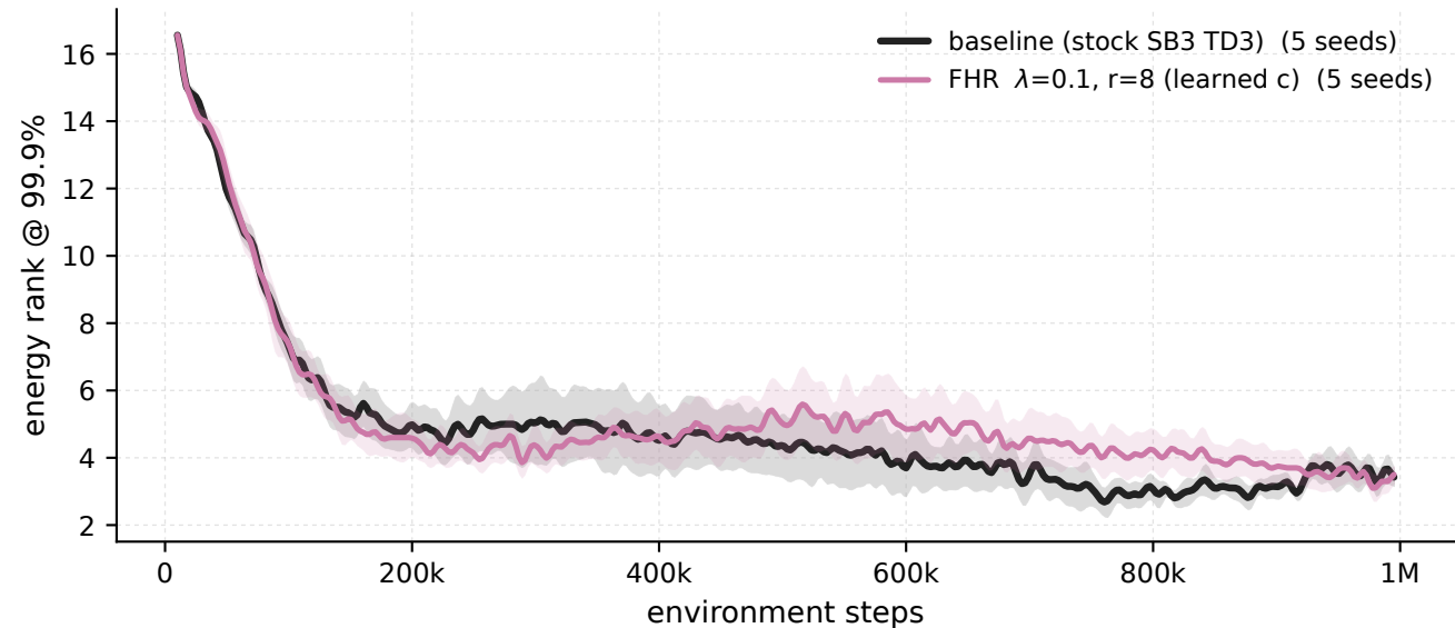
Ant-v5 - \lambda 0.1 \cdot r_8 vs baseline, penalised windows energy rank @ 99.9%
