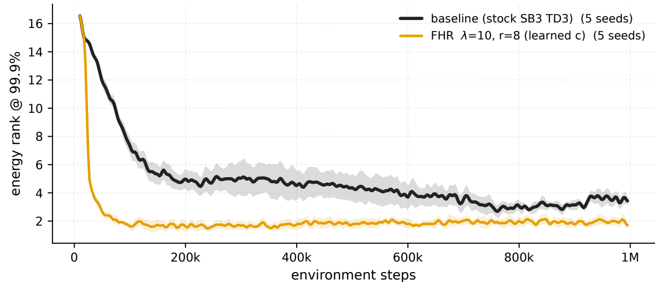
Ant-v5 - \lambda 10 \cdot r8 vs baseline, penalised windows energy rank @ 99.9%
