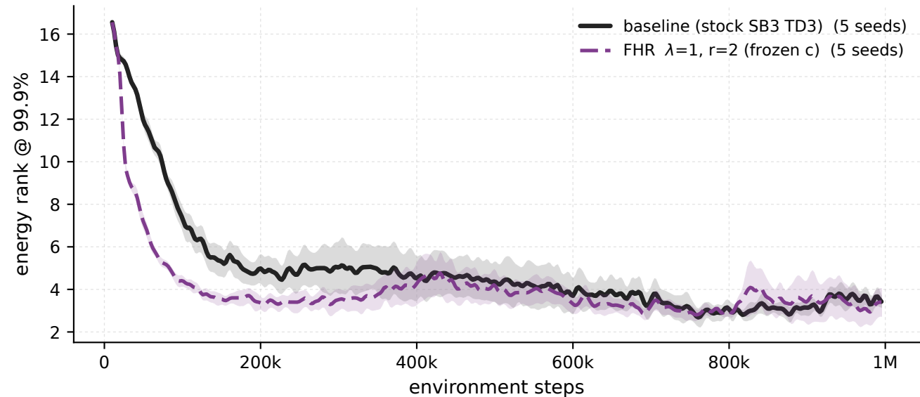
Ant-v5 - \lambda 1 \cdot r 2 frozen-c vs baseline, penalised windows energy rank @ 99.9%
