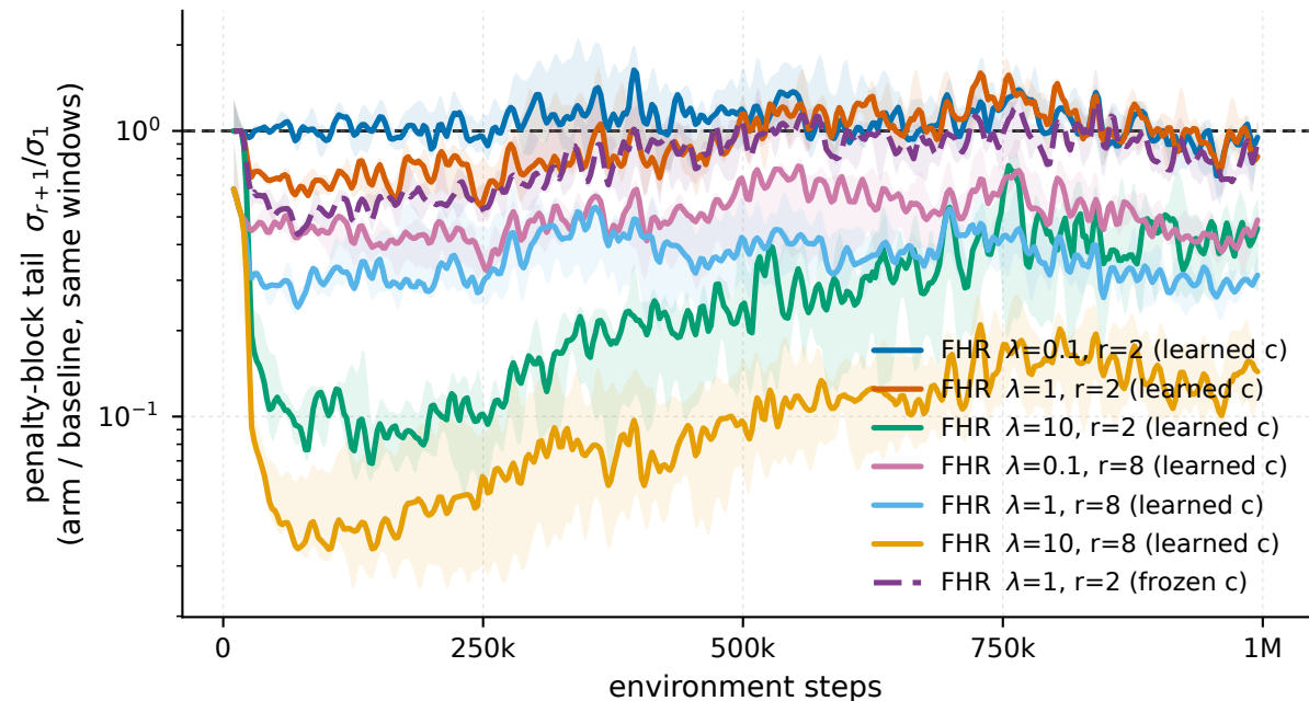
Ant-v5 - compression relative to the baseline
