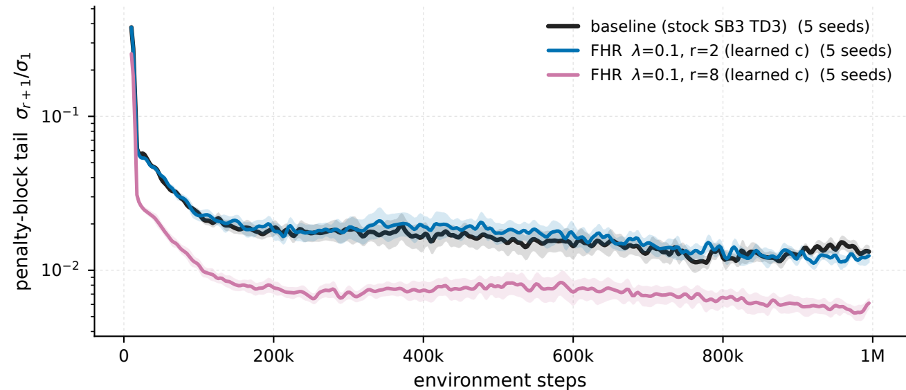
Ant-v5 - \lambda 0.1 \cdot r_2 , \lambda 0.1 \cdot r_8 vs baseline, penalised windows penalty-block tail \sigma_{r+1}/\sigma_1
