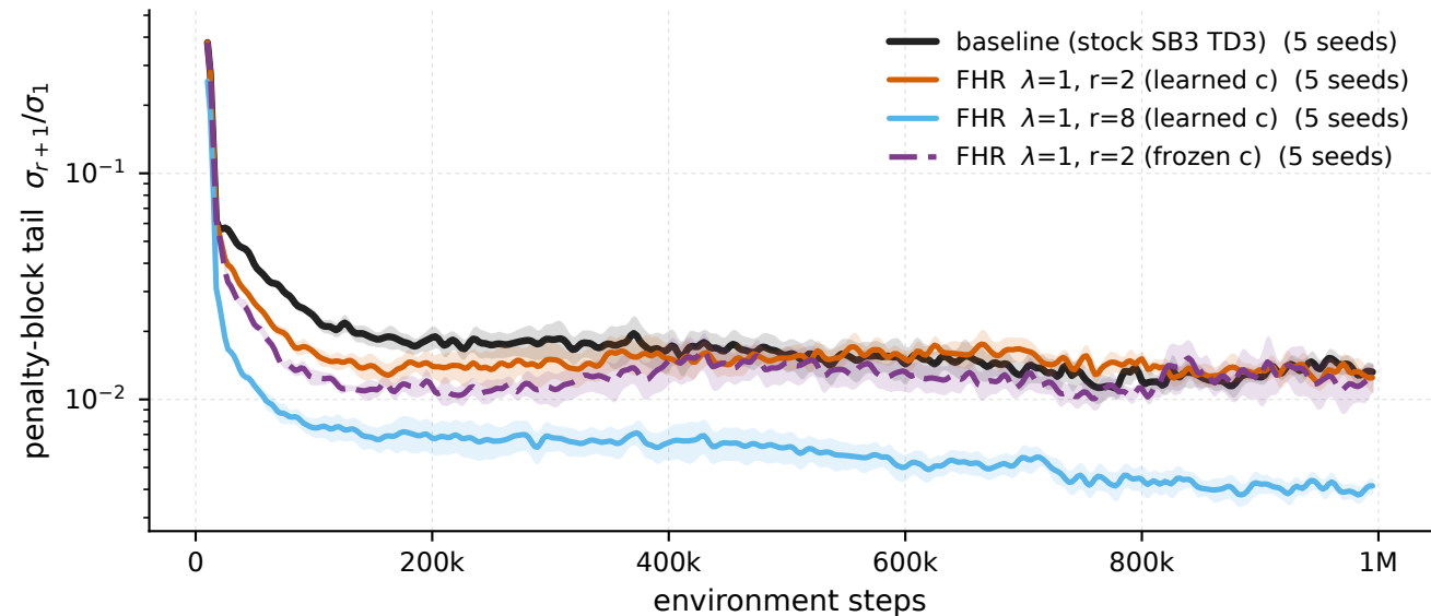
Ant-v5 - \lambda 1 \cdot r_2 , \lambda 1 \cdot r_8 , \lambda 1 \cdot r_2 frozen-c vs baseline, penalised windows penalty-block tail \sigma_{r+1}/\sigma_1
