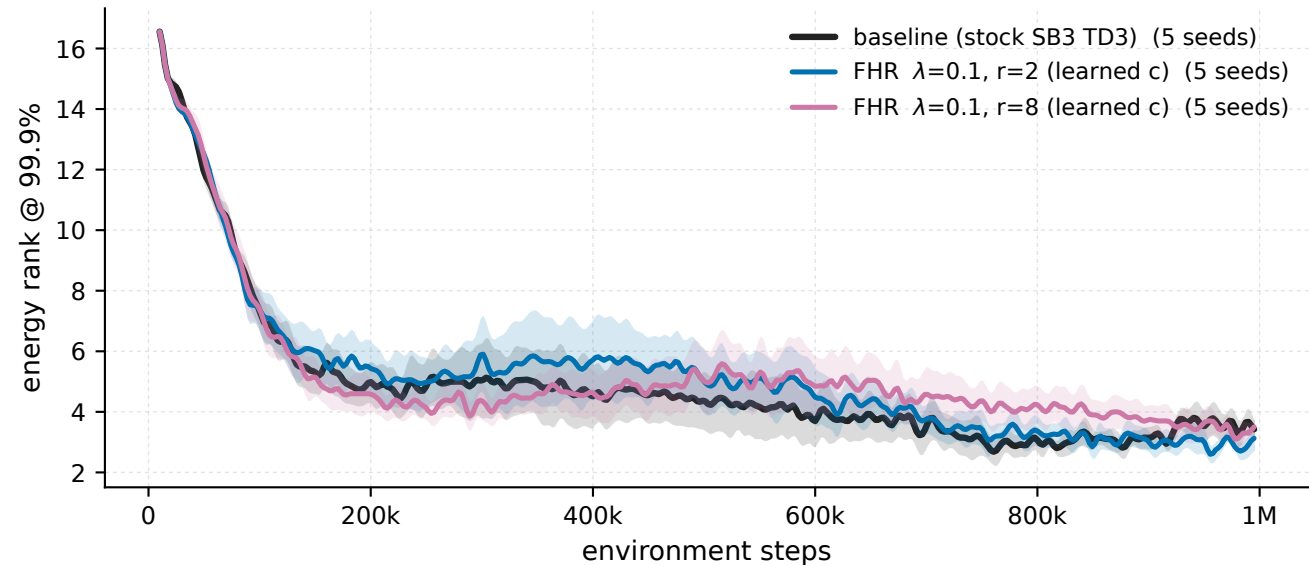
Ant-v5 - \lambda 0.1 \cdot r_2 , \lambda 0.1 \cdot r_8 vs baseline, penalised windows energy rank @ 99.9%
