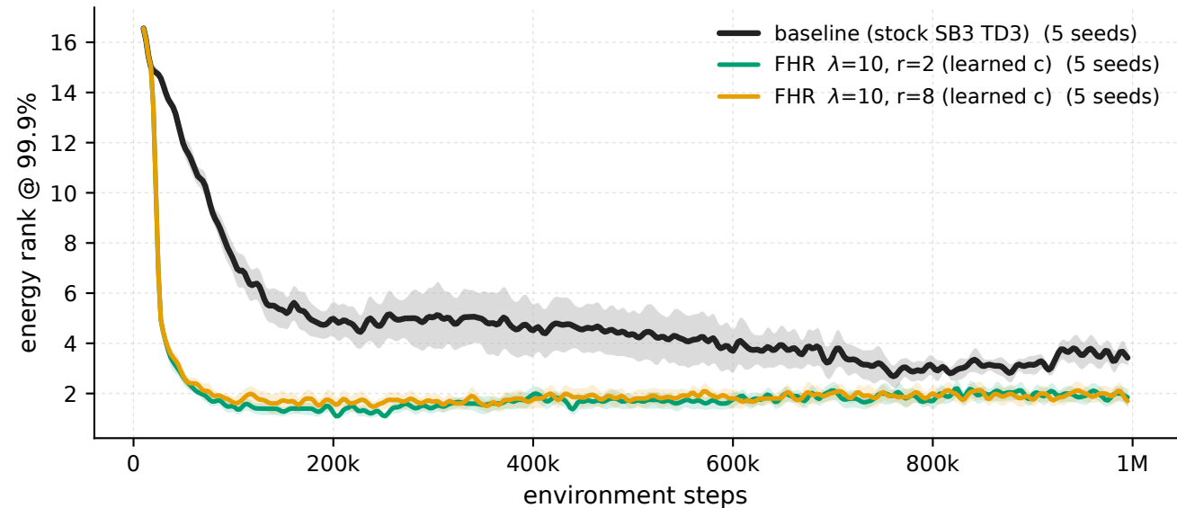
Ant-v5 - \lambda 10 \cdot r_2 , \lambda 10 \cdot r_8 vs baseline, penalised windows energy rank @ 99.9%
