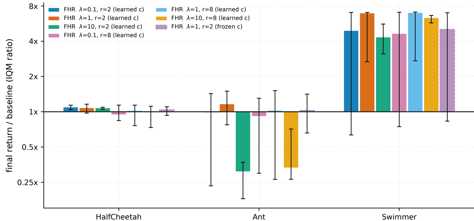
FHR arms across environments (bars: IQM ratio; whiskers: 95% bootstrap CI)
