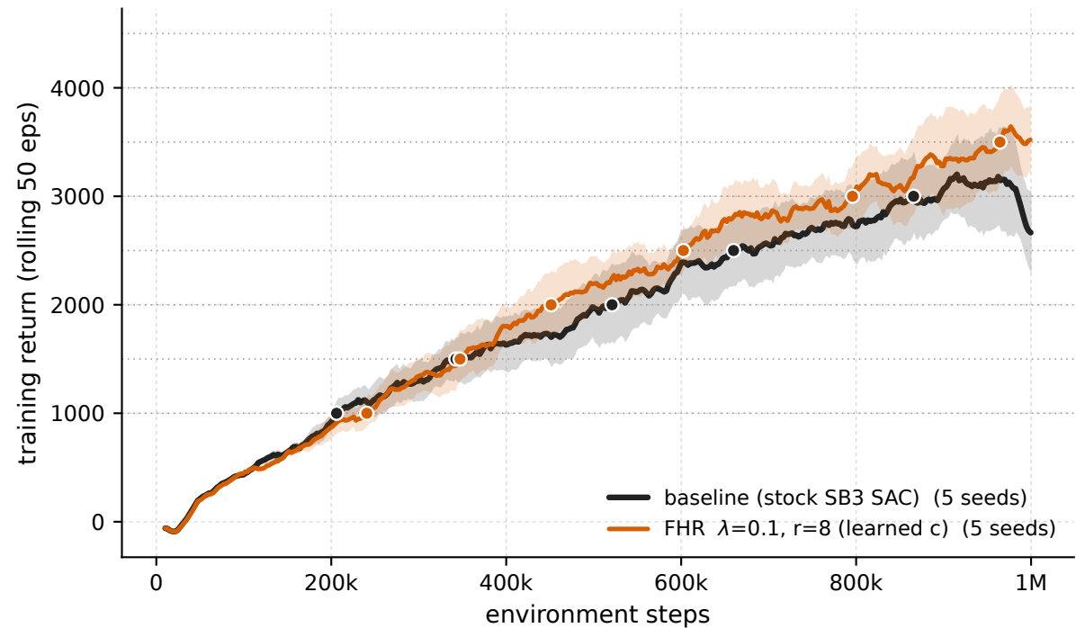
Ant-v5 - \lambda 0.1 \cdot r8 vs baseline (training stream)
