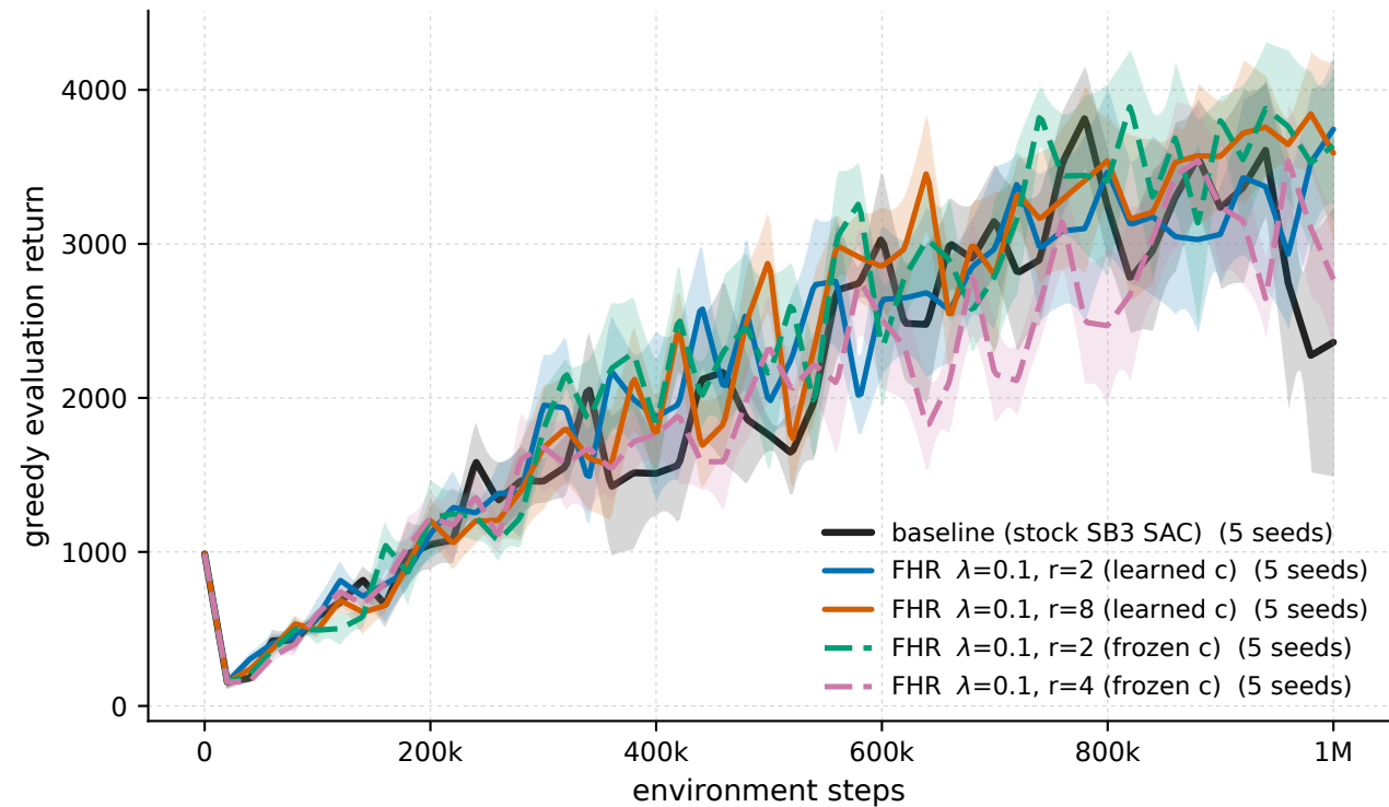
Ant-v5 - all arms (eval)
