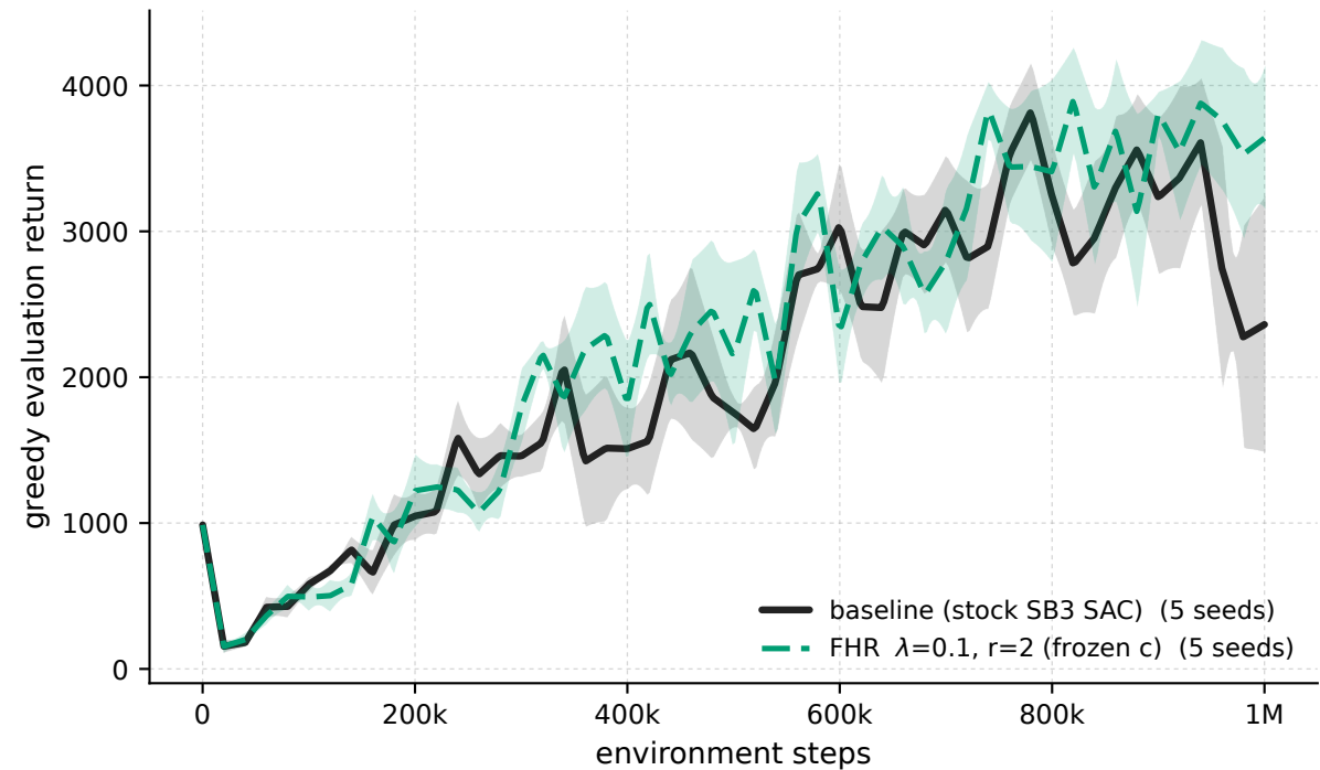
Ant-v5 - \lambda 0.1 \cdot r2 frozen-c vs baseline (greedy eval)
