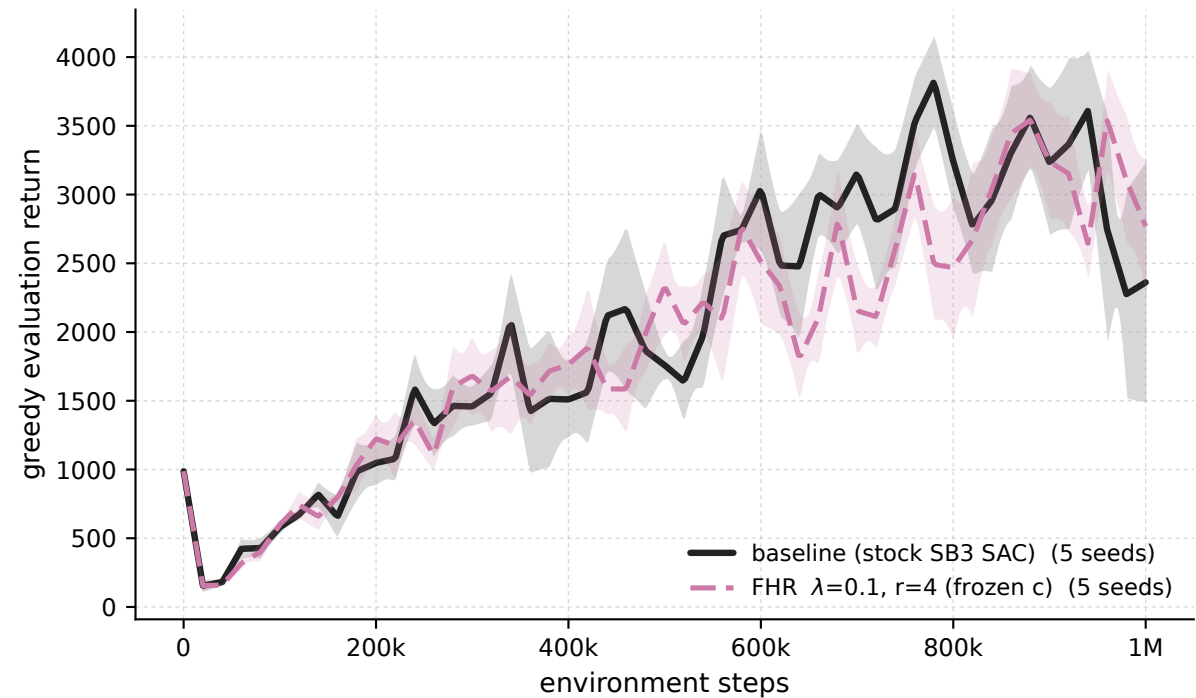
Ant-v5 - \lambda 0.1 \cdot r4 frozen-c vs baseline (greedy eval)
