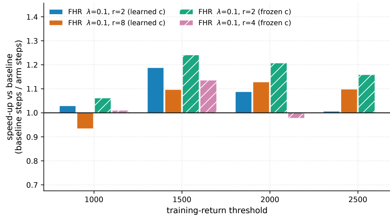
Ant-v5 - sample-efficiency ratio (thresholds all baseline seeds reached)
