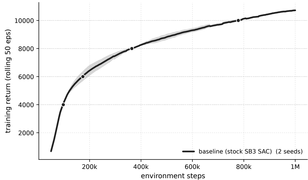
HalfCheetah-v5 - \lambda 0.1 \cdot r_2 vs baseline (training stream)
