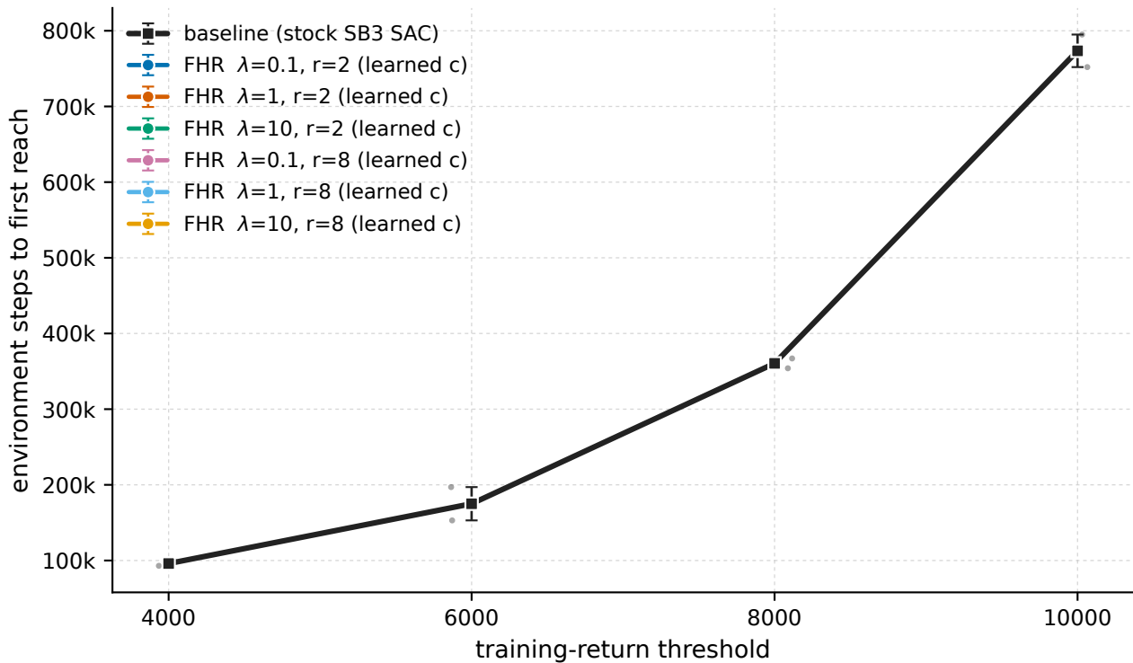
HalfCheetah-v5 - sample efficiency, training stream (mean \pm 1 s.e.m.)
