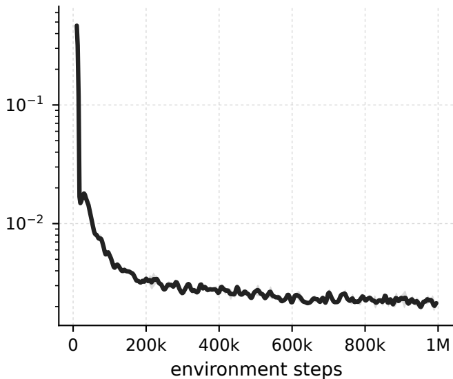
HalfCheetah-v5 - \lambda 10 \cdot r_8 vs baseline, penalised-window Hankel spectrum energy rank @ 99.9%
