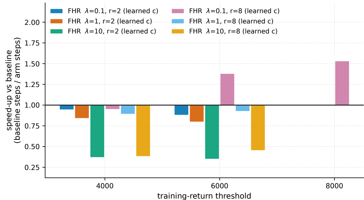
HalfCheetah-v5 - sample-efficiency ratio (thresholds all baseline seeds reached)
