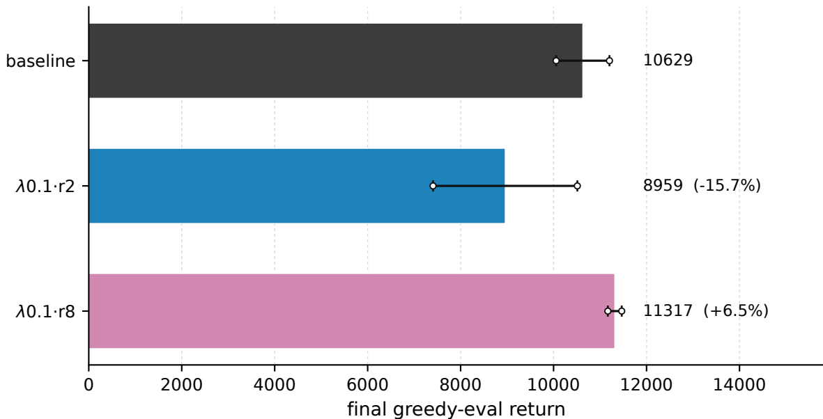
HalfCheetah-v5 - final return, \lambda = 0.1 vs baseline
