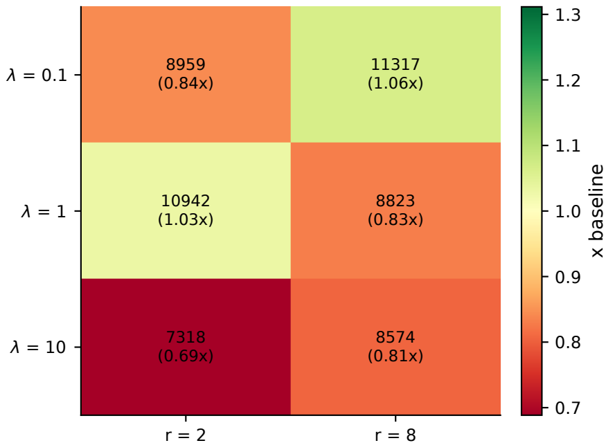
final return vs baseline (10629)
