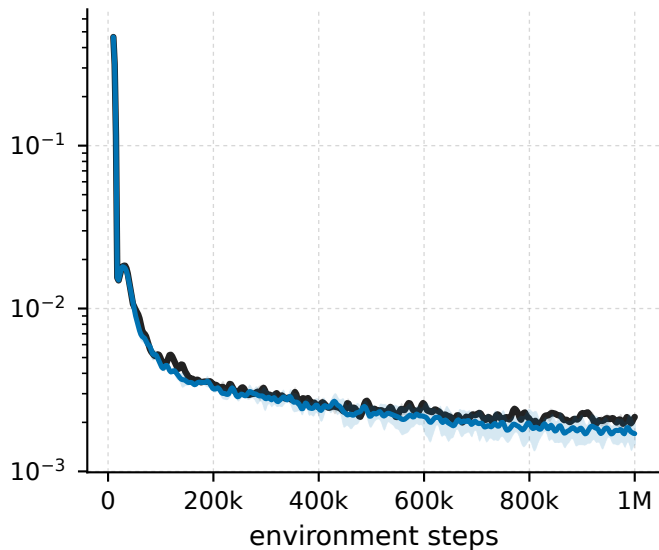
HalfCheetah-v5 - \lambda 0.1 \cdot r_2 vs baseline, penalised-window Hankel spectrum energy rank @ 99.9%
