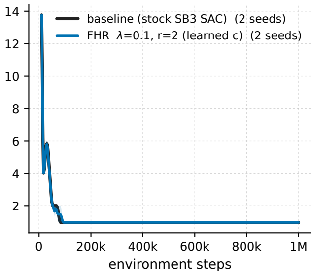
HalfCheetah-v5 - \lambda 0.1 \cdot r_2 vs baseline, penalised-window Hankel spectrum energy rank @ 99.9%
