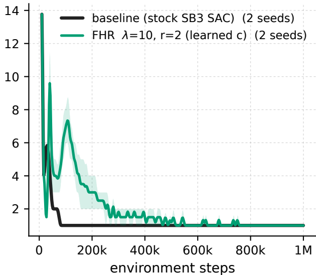
HalfCheetah-v5 - \lambda 10 \cdot r_2 vs baseline, penalised-window Hankel spectrum energy rank @ 99.9% penalty-block tail \sigma_{r+1}/\sigma_1
