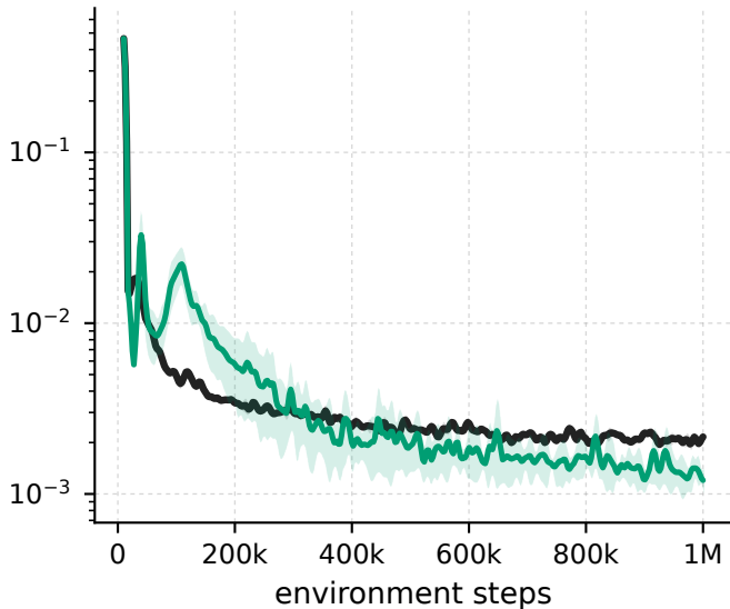
HalfCheetah-v5 - \lambda 10 \cdot r_2 vs baseline, penalised-window Hankel spectrum energy rank @ 99.9% penalty-block tail \sigma_{r+1}/\sigma_1
