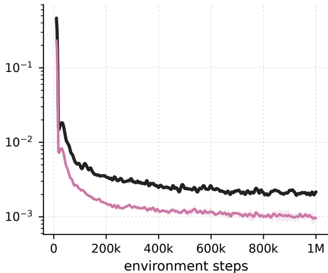
HalfCheetah-v5 - \lambda 0.1 \cdot r_8 vs baseline, penalised-window Hankel spectrum energy rank @ 99.9%
