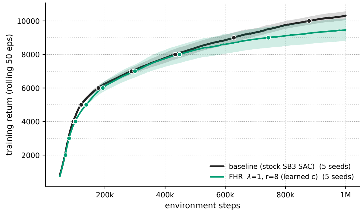
HalfCheetah-v5 - \lambda 1 \cdot r8 vs baseline (training stream)
