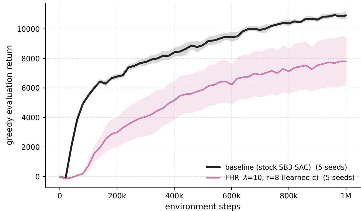
HalfCheetah-v5 - \lambda 10 \cdot r8 vs baseline (greedy eval)
