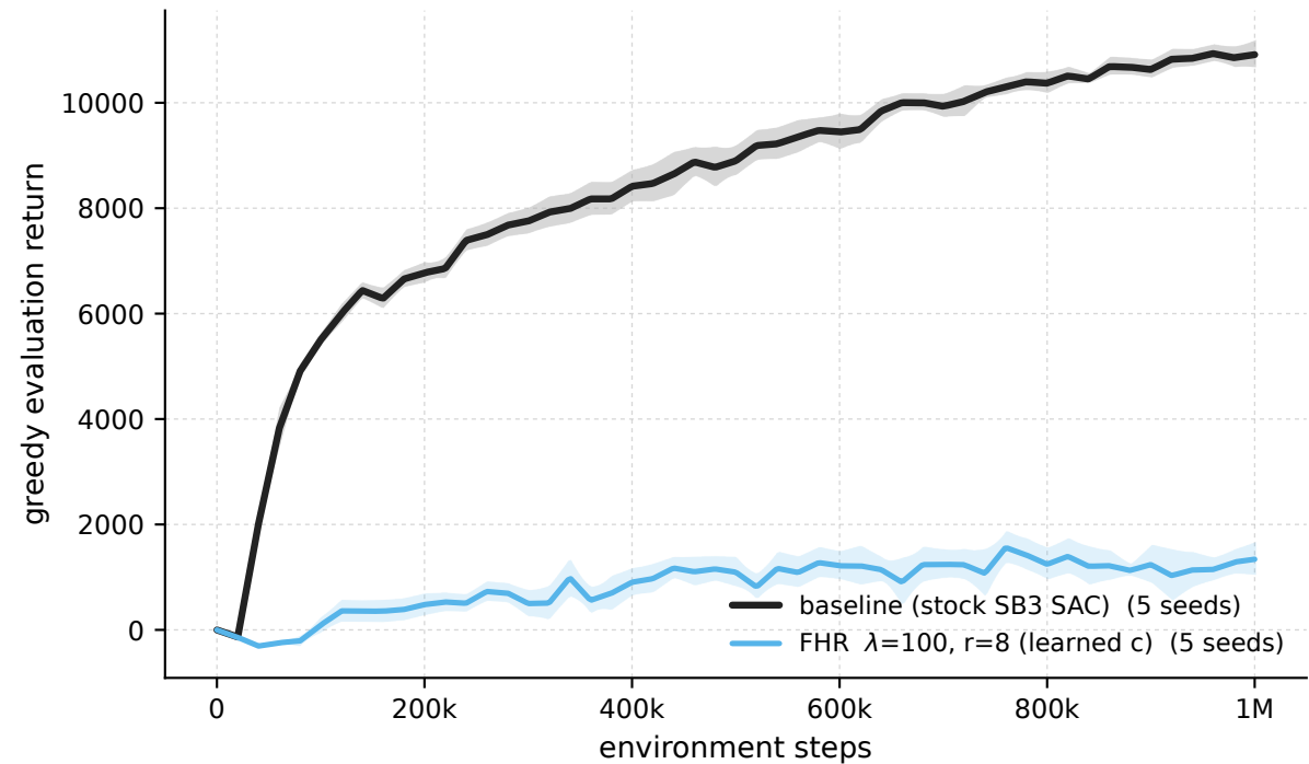
HalfCheetah-v5 - \lambda 100 \cdot r8 vs baseline (greedy eval)
