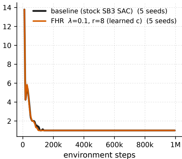
HalfCheetah-v5 - \lambda 0.1 \cdot r_8 vs baseline, penalised-window Hankel spectrum energy rank @ 99.9%
