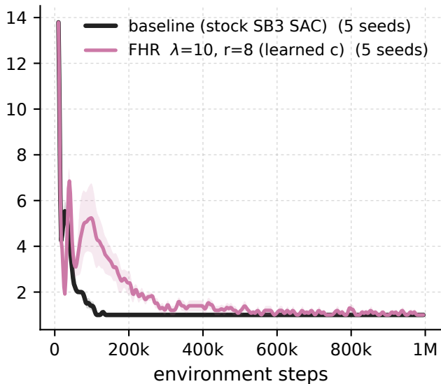
HalfCheetah-v5 - \lambda 10 \cdot r8 vs baseline, penalised-window Hankel spectrum energy rank @ 99.9% penalty-block tail \sigma_{r+1}/\sigma_1
