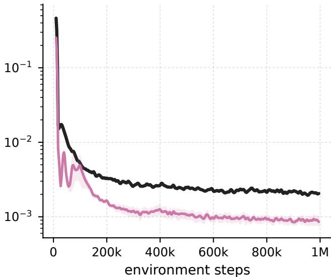
HalfCheetah-v5 - \lambda 10 \cdot r8 vs baseline, penalised-window Hankel spectrum energy rank @ 99.9% penalty-block tail \sigma_{r+1}/\sigma_1
