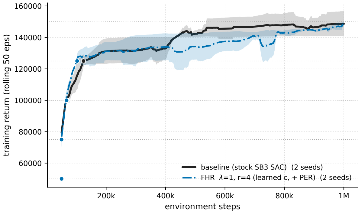
HumanoidStandup-v5 - \lambda 1 \cdot r4 +PER vs baseline (training stream)
