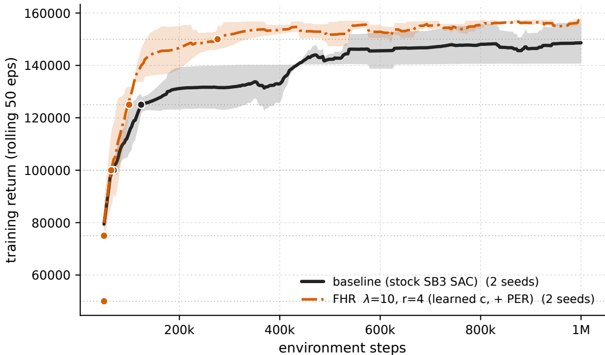
HumanoidStandup-v5 - \lambda 10 \cdot r_4 +PER vs baseline (training stream)
