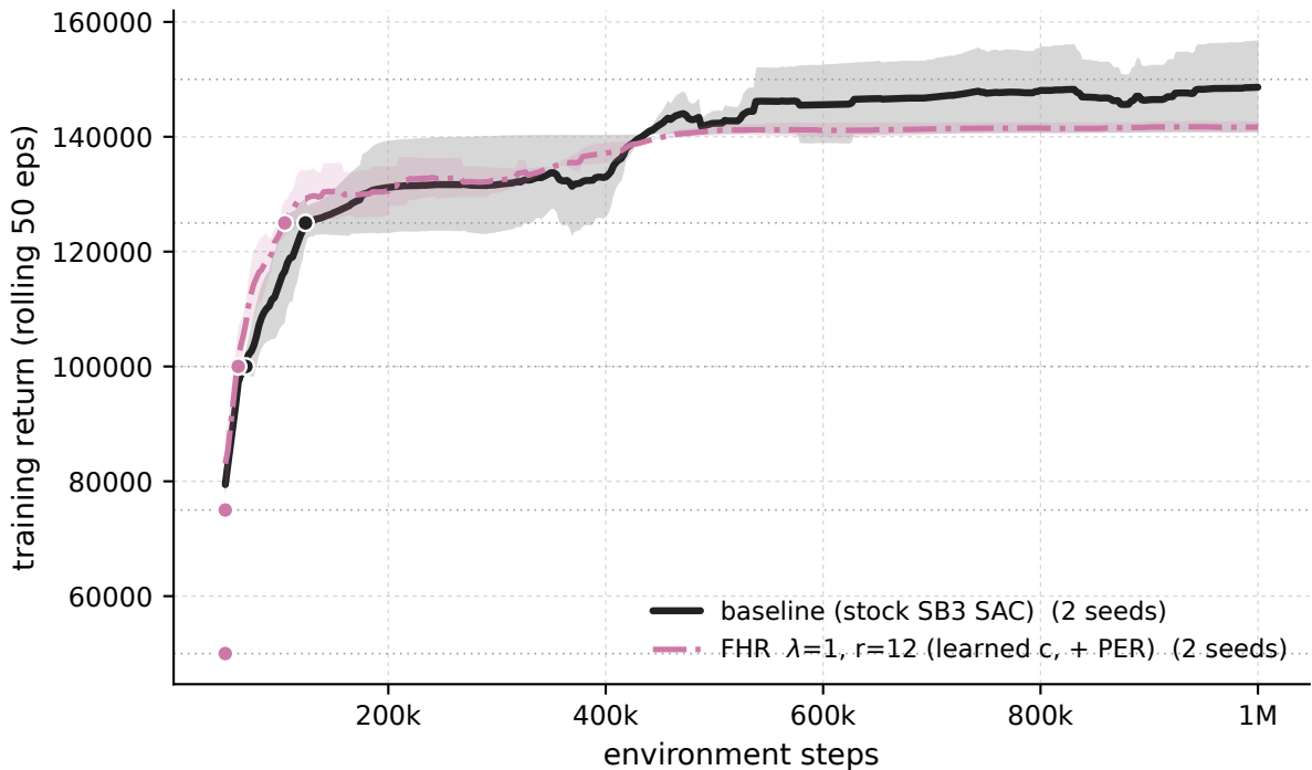
HumanoidStandup-v5 - \lambda 1 \cdot r_{12} +PER vs baseline (training stream)
