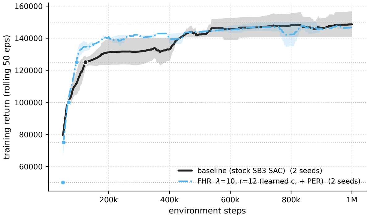
HumanoidStandup-v5 - \lambda 10 \cdot r 12 +PER vs baseline (training stream)
