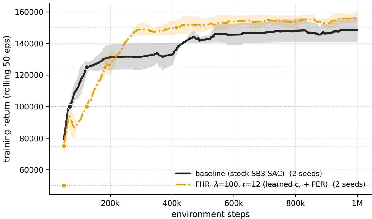
HumanoidStandup-v5 - \lambda 100 \cdot r_{12} + PER vs baseline (training stream)
