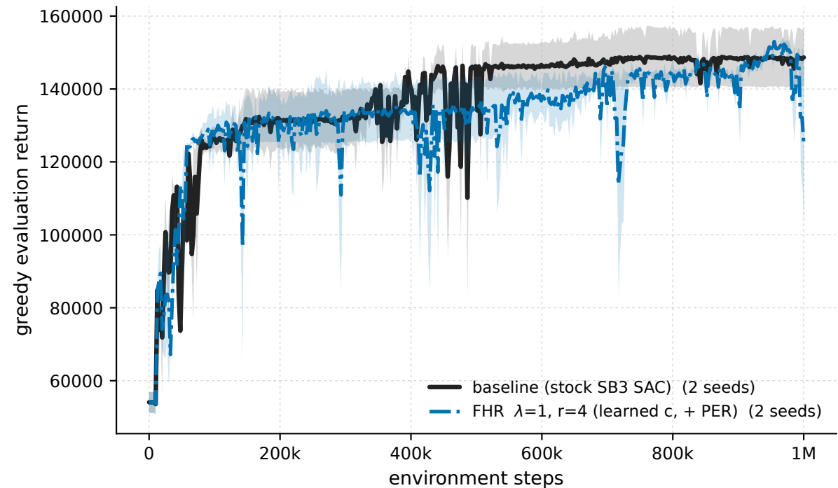
HumanoidStandup-v5 - \lambda 1 \cdot r4 +PER vs baseline (greedy eval)
