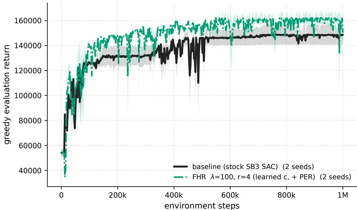
HumanoidStandup-v5 - \lambda 100 \cdot r4 +PER vs baseline (greedy eval)
