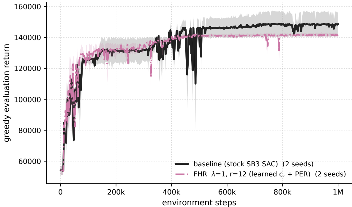
HumanoidStandup-v5 - \lambda 1 \cdot r_{12} +PER vs baseline (greedy eval)
