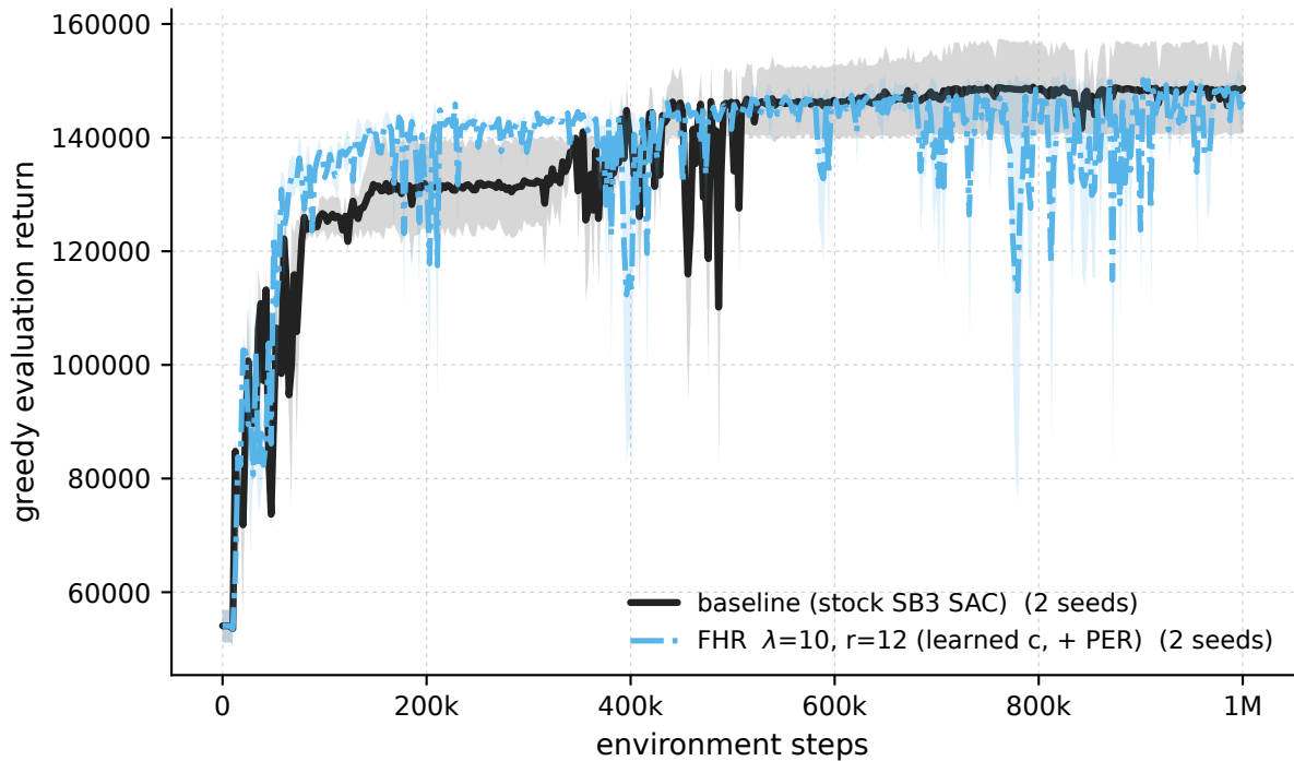
HumanoidStandup-v5 - \lambda 10 \cdot r_{12} +PER vs baseline (greedy eval)
