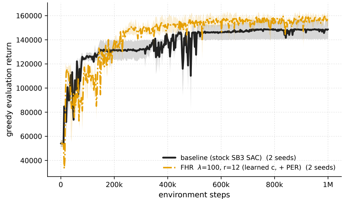
HumanoidStandup-v5 - \lambda 100 \cdot r_{12} +PER vs baseline (greedy eval)
