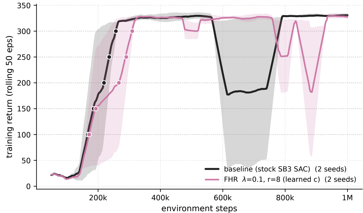
Swimmer-v5 - \lambda 0.1 \cdot r8 vs baseline (training stream)
