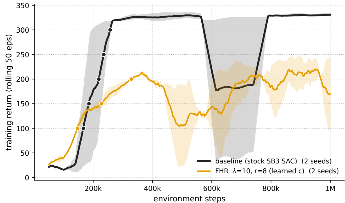
Swimmer-v5 - \lambda 10 \cdot r8 vs baseline (training stream)
