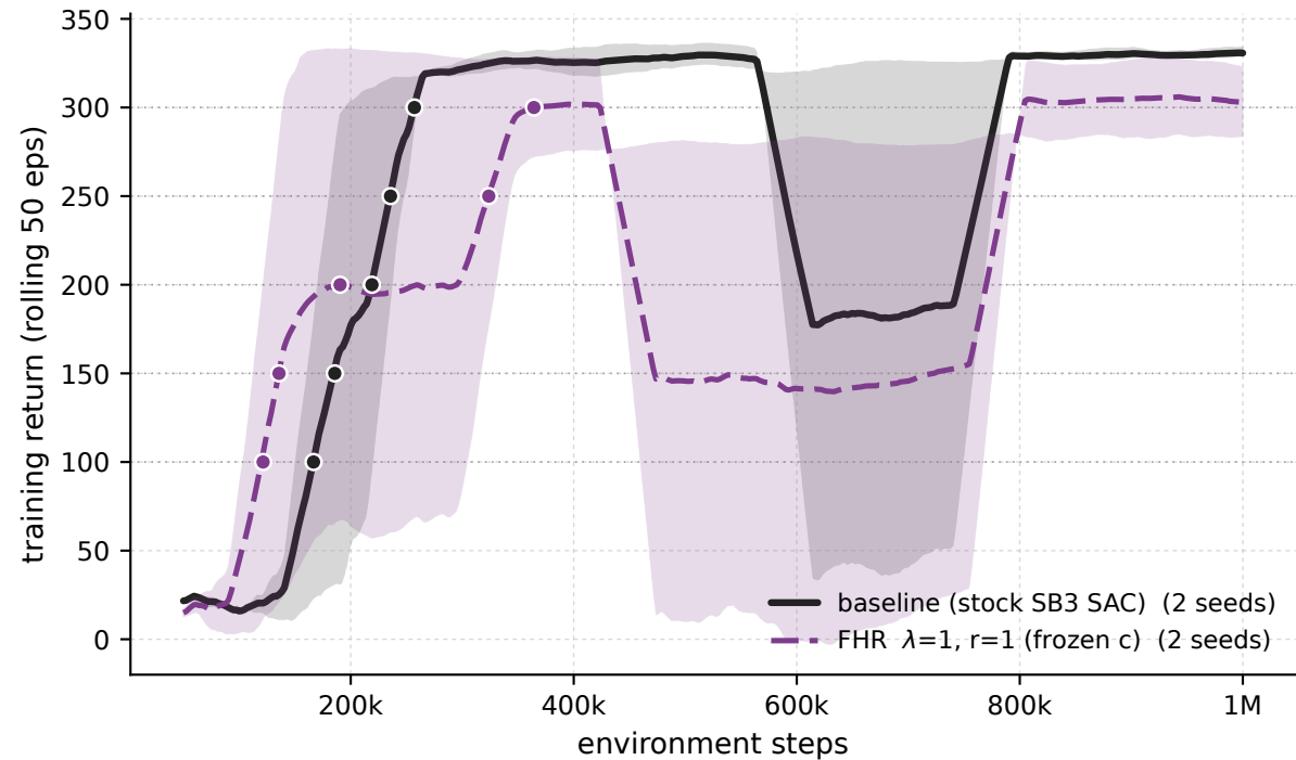
Swimmer-v5 - \lambda 1 \cdot r1 frozen-c vs baseline (training stream)
