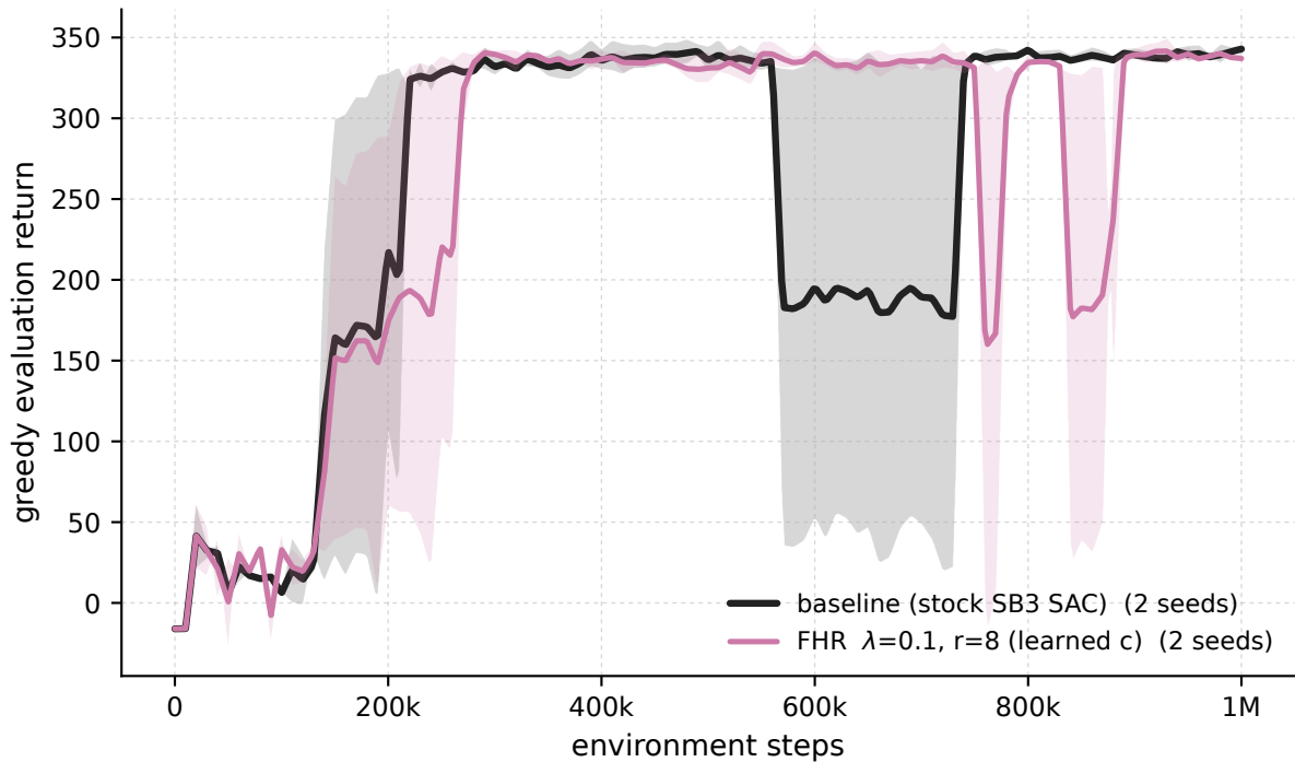
Swimmer-v5 - \lambda 0.1 \cdot r8 vs baseline (greedy eval)
