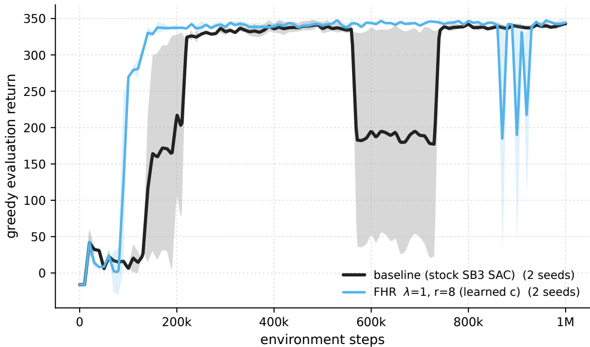
Swimmer-v5 - \lambda 1 \cdot r8 vs baseline (greedy eval)
