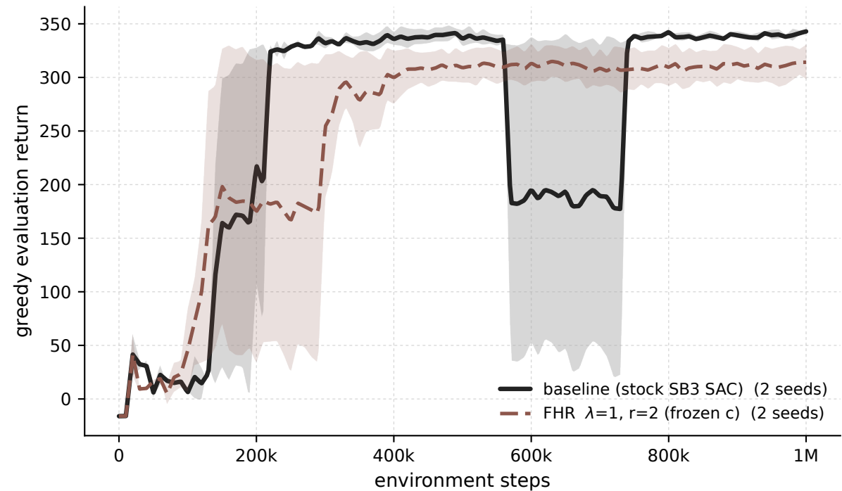
Swimmer-v5 - \lambda 1 \cdot r2 frozen-c vs baseline (greedy eval)
