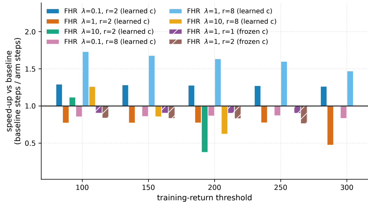
Swimmer-v5 - sample-efficiency ratio (thresholds all baseline seeds reached)
