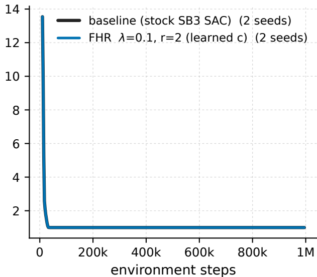
Swimmer-v5 - \lambda 0.1 \cdot r^2 vs baseline, penalised-window Hankel spectrum energy rank @ 99.9%
