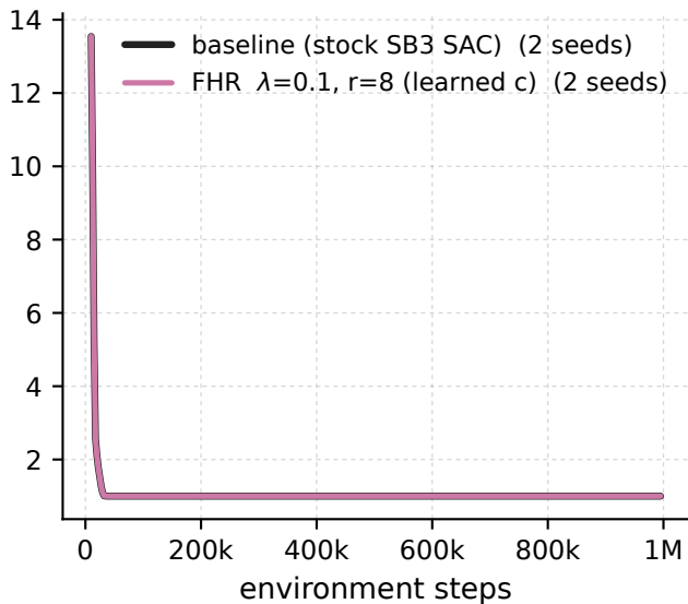
Swimmer-v5 - \lambda 0.1 \cdot r8 vs baseline, penalised-window Hankel spectrum energy rank @ 99.9%
