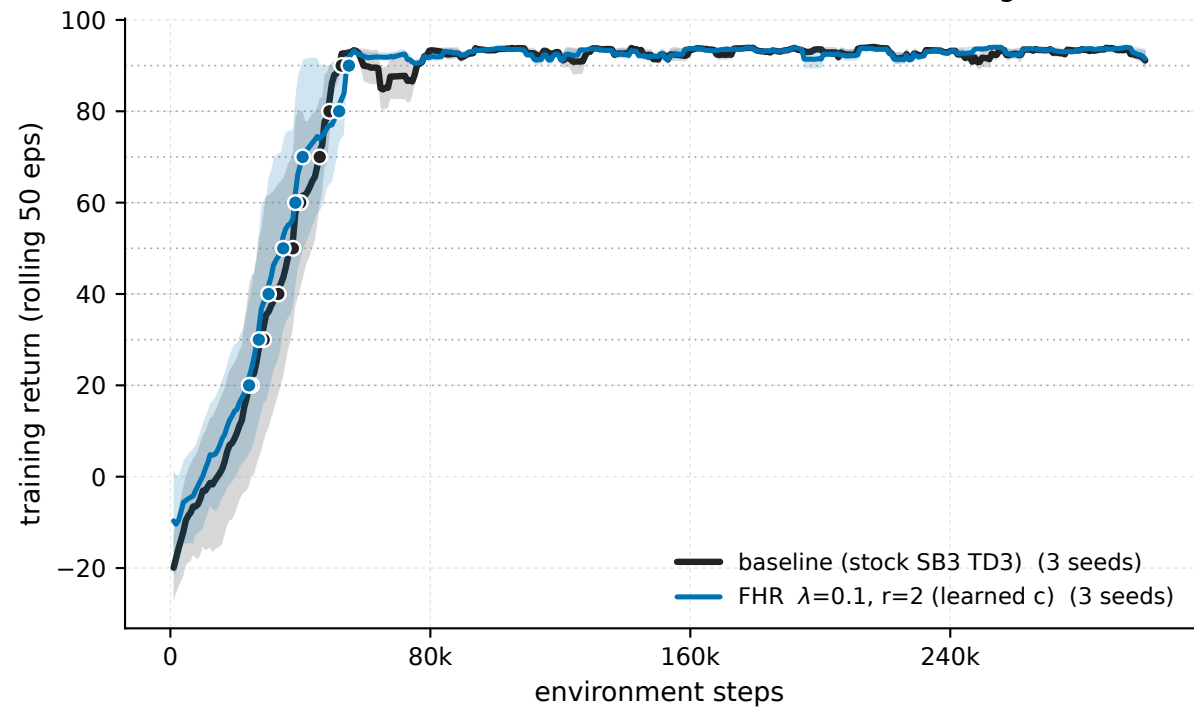
MountainCarContinuous-v0 - \lambda 0.1 \cdot r_2 vs baseline (training stream)
